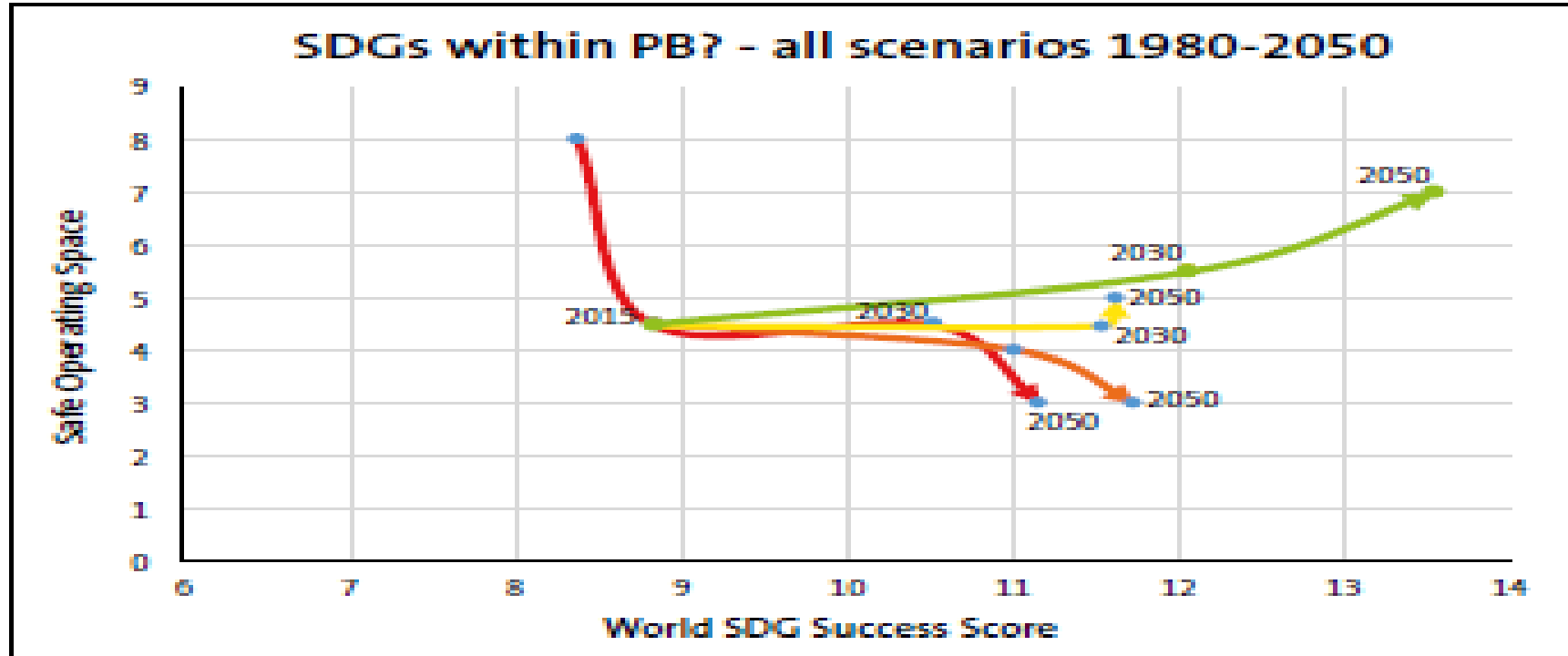
Figure 1.7 Achieving the SDGs within PBs: Only one of the four scenarios achieves the grand challenge of improving the world's SDG Success Score, without eroding Earth's Safety Margin.
